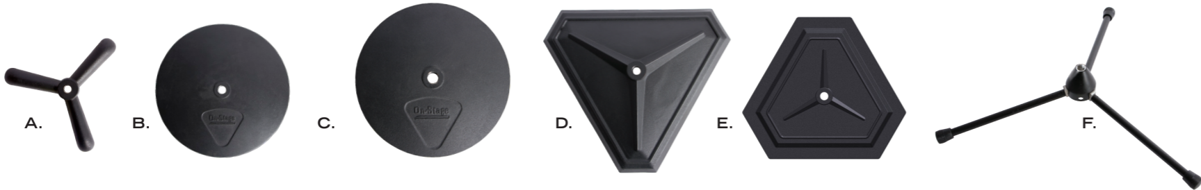
A. 5 lb. Sand-cast Tripod Base / BA7311 / 13124 B. 10" Round Base / BA1006 / 13112 C. 12" Round Base / BA1210 / 13123 D. 16 lb. Hex Base / BA1516 / 13125 E. 13.25 lb. Hex Base / BA1313 / 13092 F. Heavy-Duty Tripod Base / BA9750 / 13154
